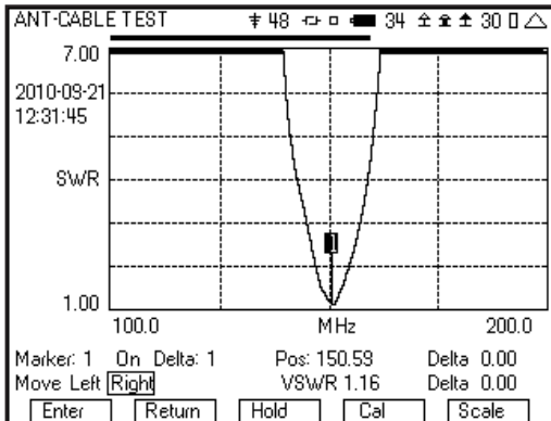
VSWR of a VHF Antenna
